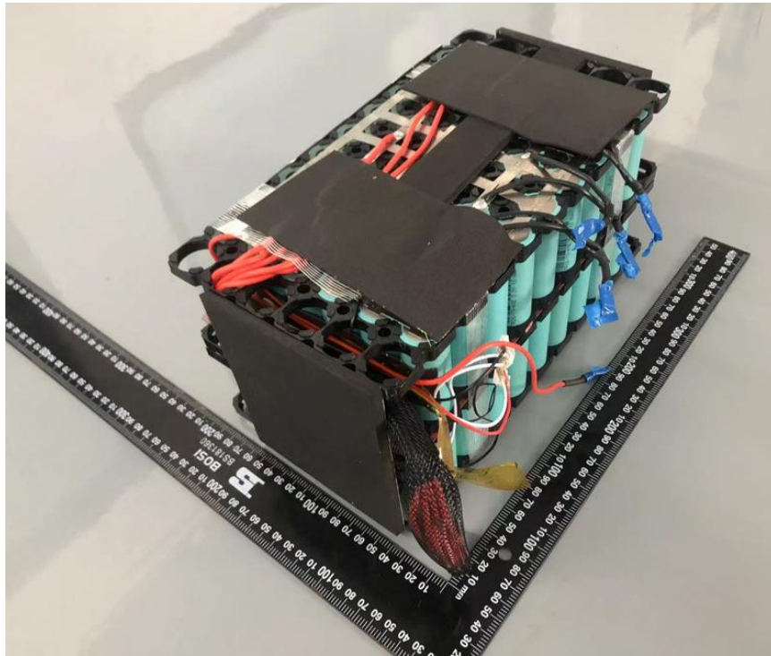
Internal View 2
