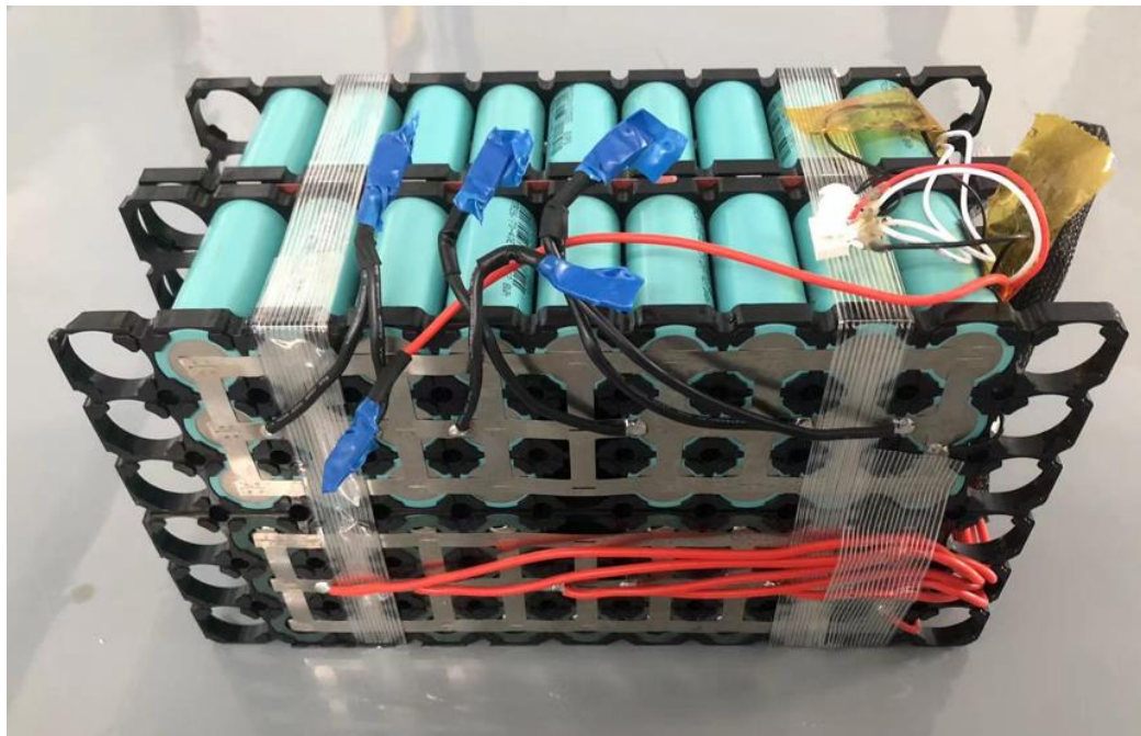
Internal View 3
