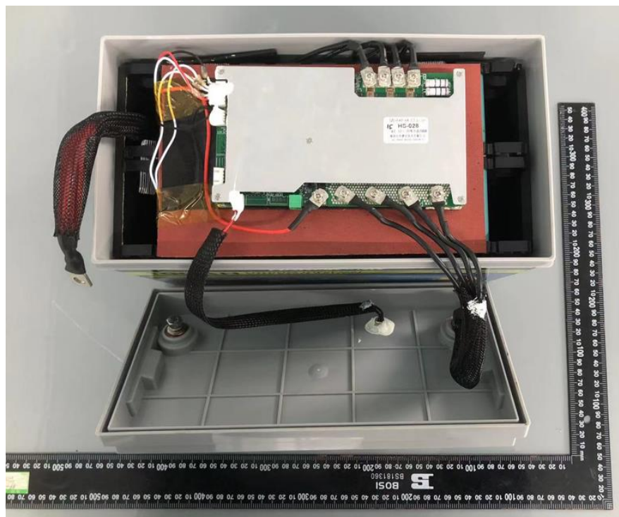
Internal View 1
